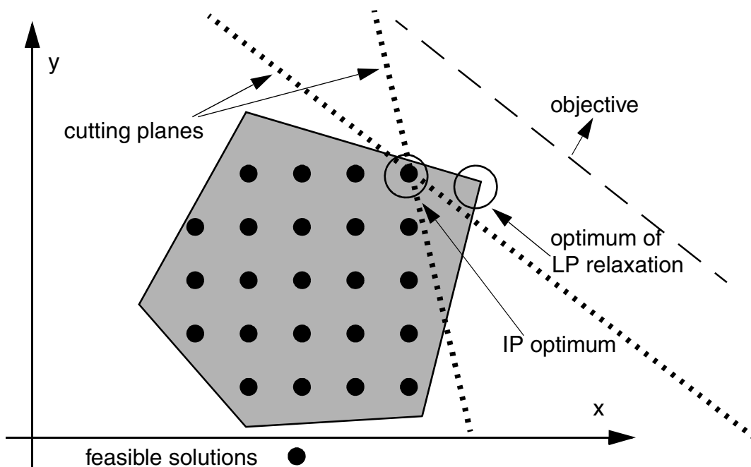
Figure 28.1 Cuts in a typical MIP
