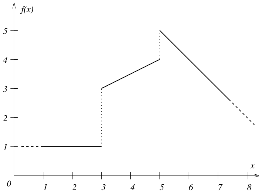
Figure 18.2 A discontinuous piecewise linear function with steps
