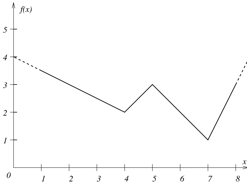
Figure 18.1 A piecewise linear function with breakpoints
