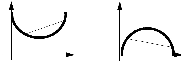
Figure 12.1 Minimize a Convex Objective Function, Maximize a Concave Objective Function
