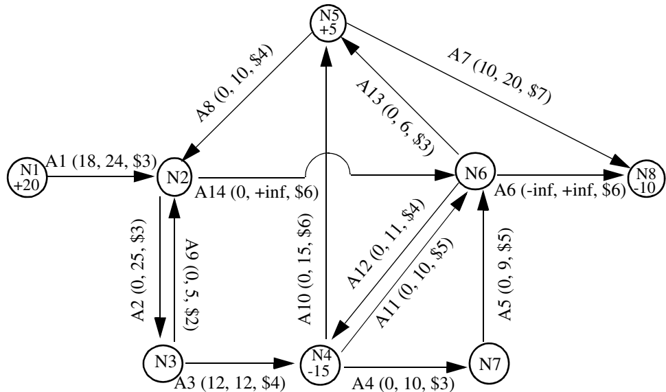
Figure 11.1 A Directed Network with Arc-Capacity, Flow-Cost, Sinks, and Sources
