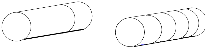
Figure 23.1 Two different patterns from a roll of stock
