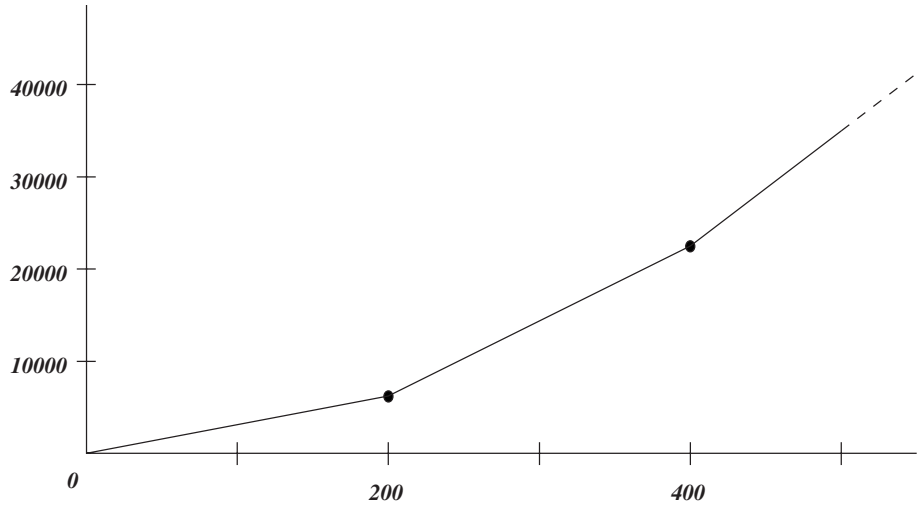
Figure 18.4 A convex piecewise linear cost function
