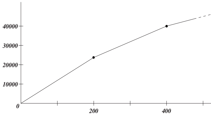
Figure 18.3 A concave piecewise linear cost function
